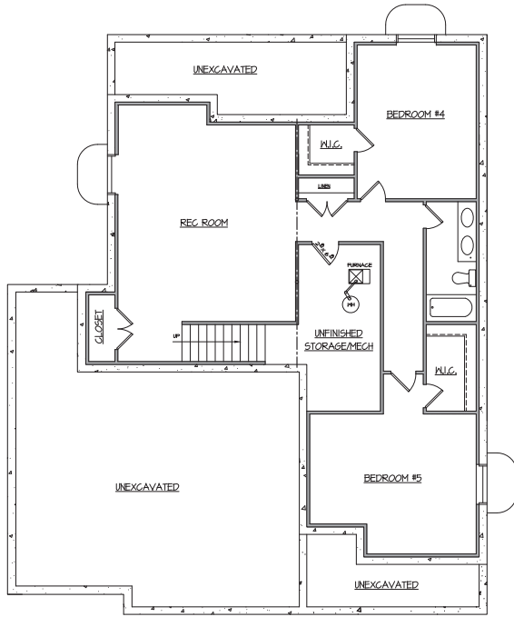
BASEMENT PLAN
